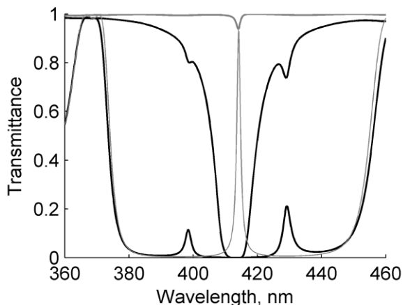
Fig.3. Transmission spectrum of the structure for the waves of left and right circular polarizations at a concentration of nanoparticles f = 0 - grey line, f = 0.02 - black line.
